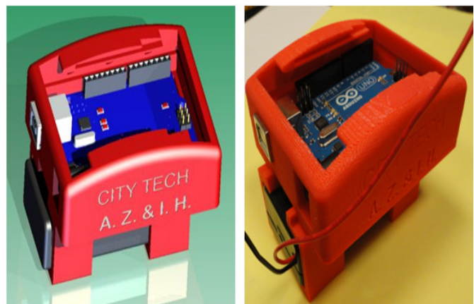
Figure 7. Computer Rendering and Physical Prototype of the AirCasting Device
