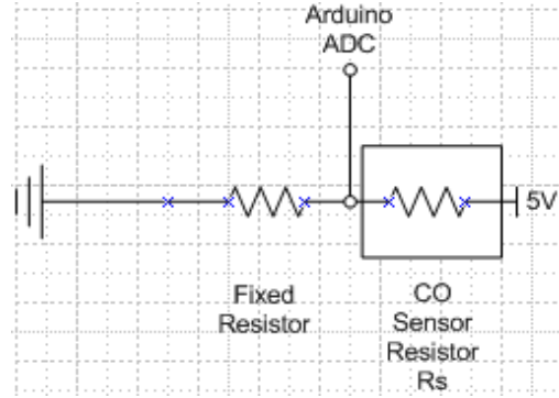
Figure 4. CO Sensor Resistor
